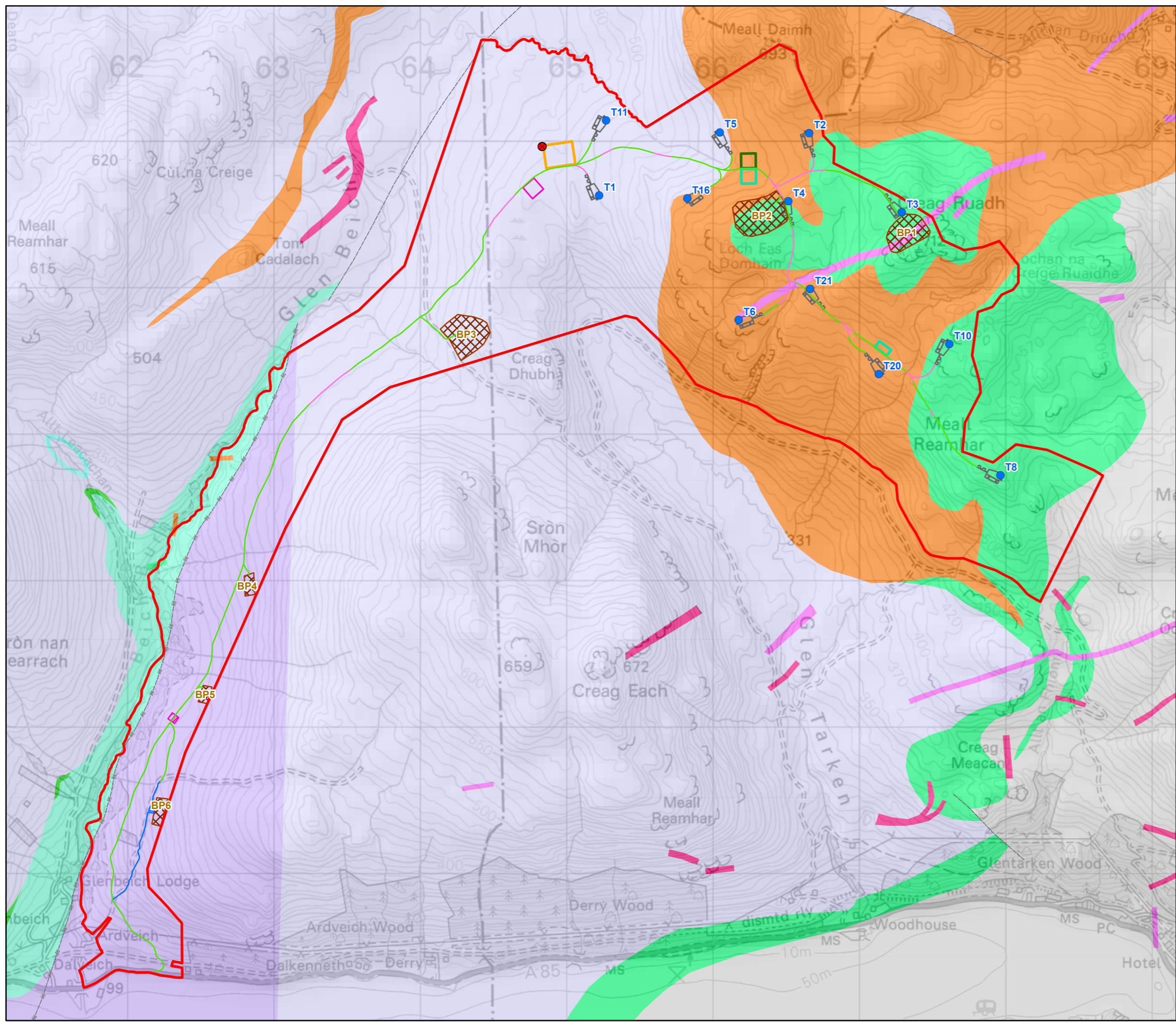
Figure 8.1.4a Peat Landslide and Hazard Risk Assessment: Bedrock Geology Glentarken Wind Farm EIAR 2024
