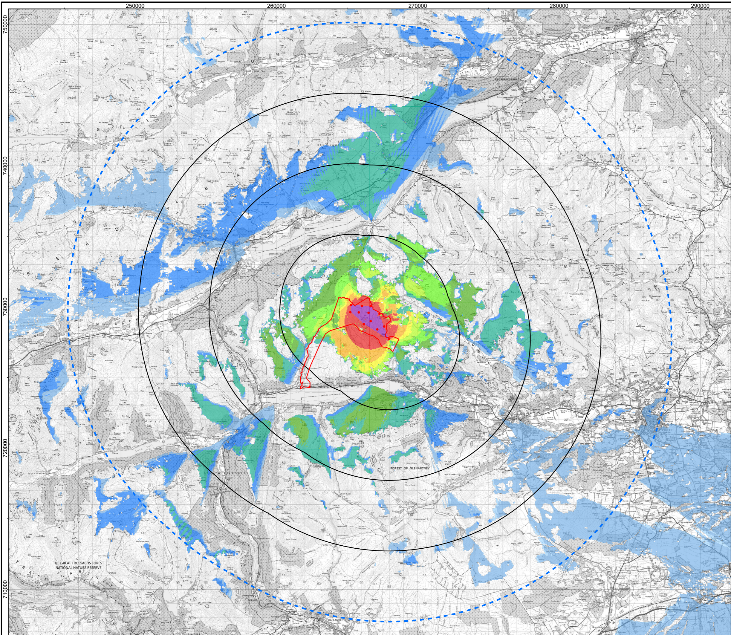
Figure 5.9 Horizontal Angle Blade Tip ZTV Glentarken Wind Farm EIAR 2024
