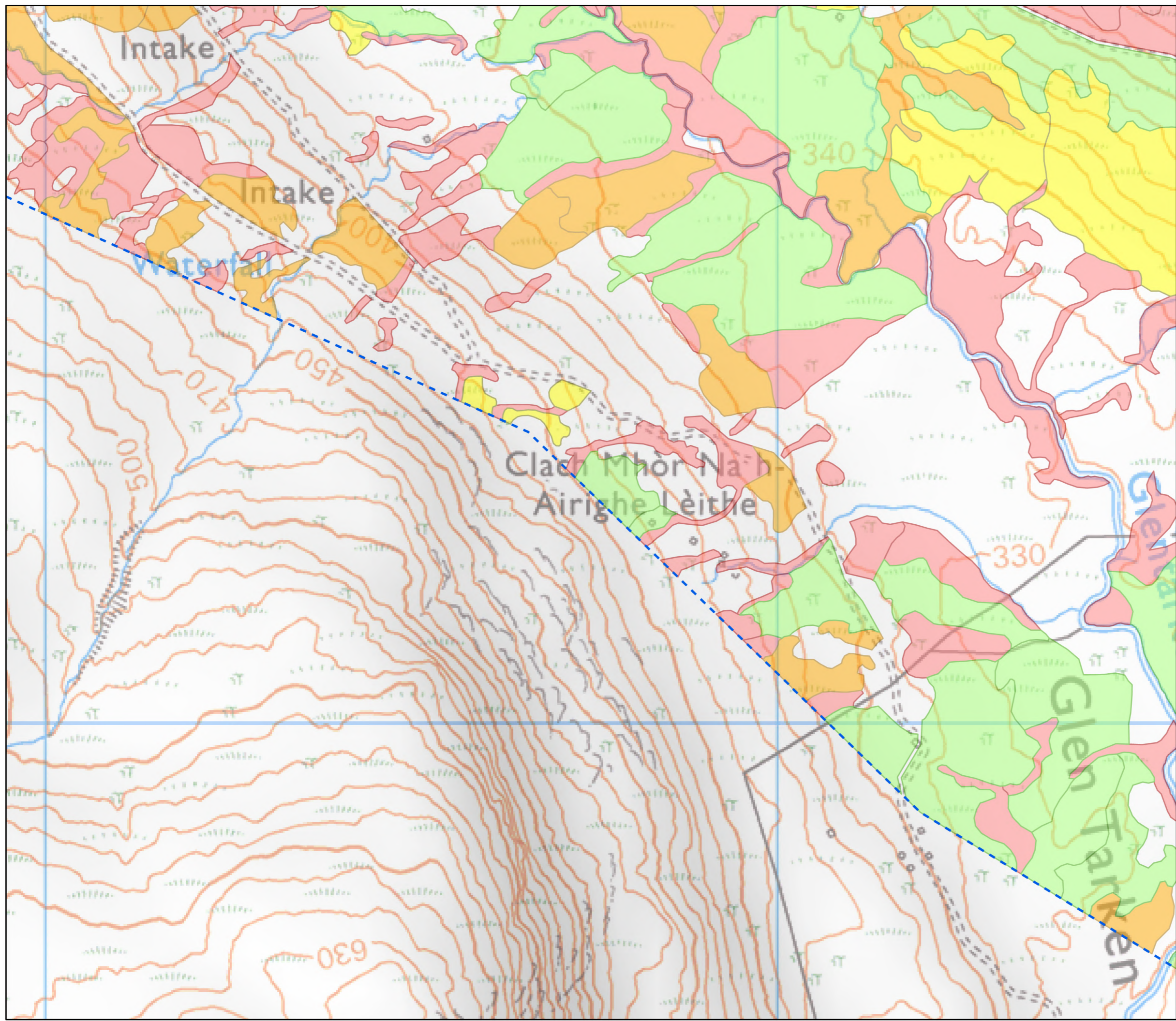
Figure 7.4.8 Potential Groundwater Dependent Terrestrial Ecosystems (GWDTEs) Glentarken Wind Farm EIAR 2024
