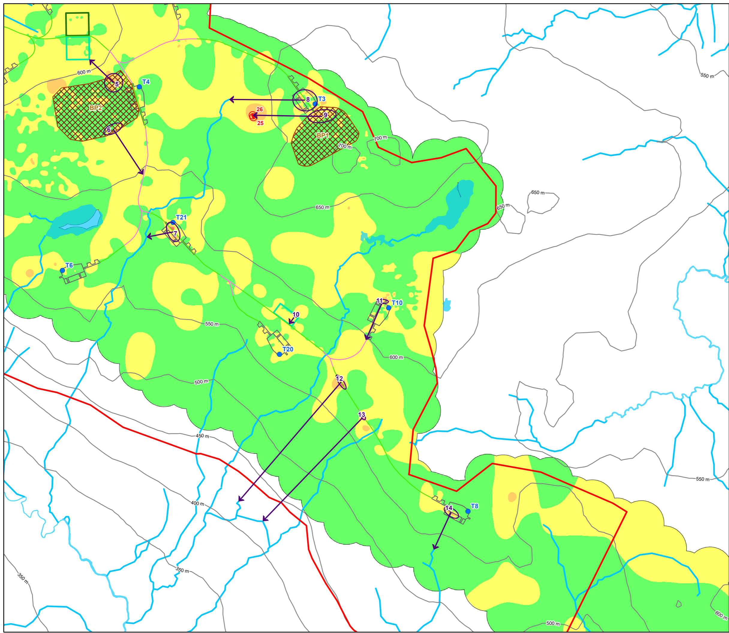
Figure 8.1.9.5 Peat Landslide and Hazard Risk Assessment: Slide Risk Glentarken Wind Farm EIAR 2024
