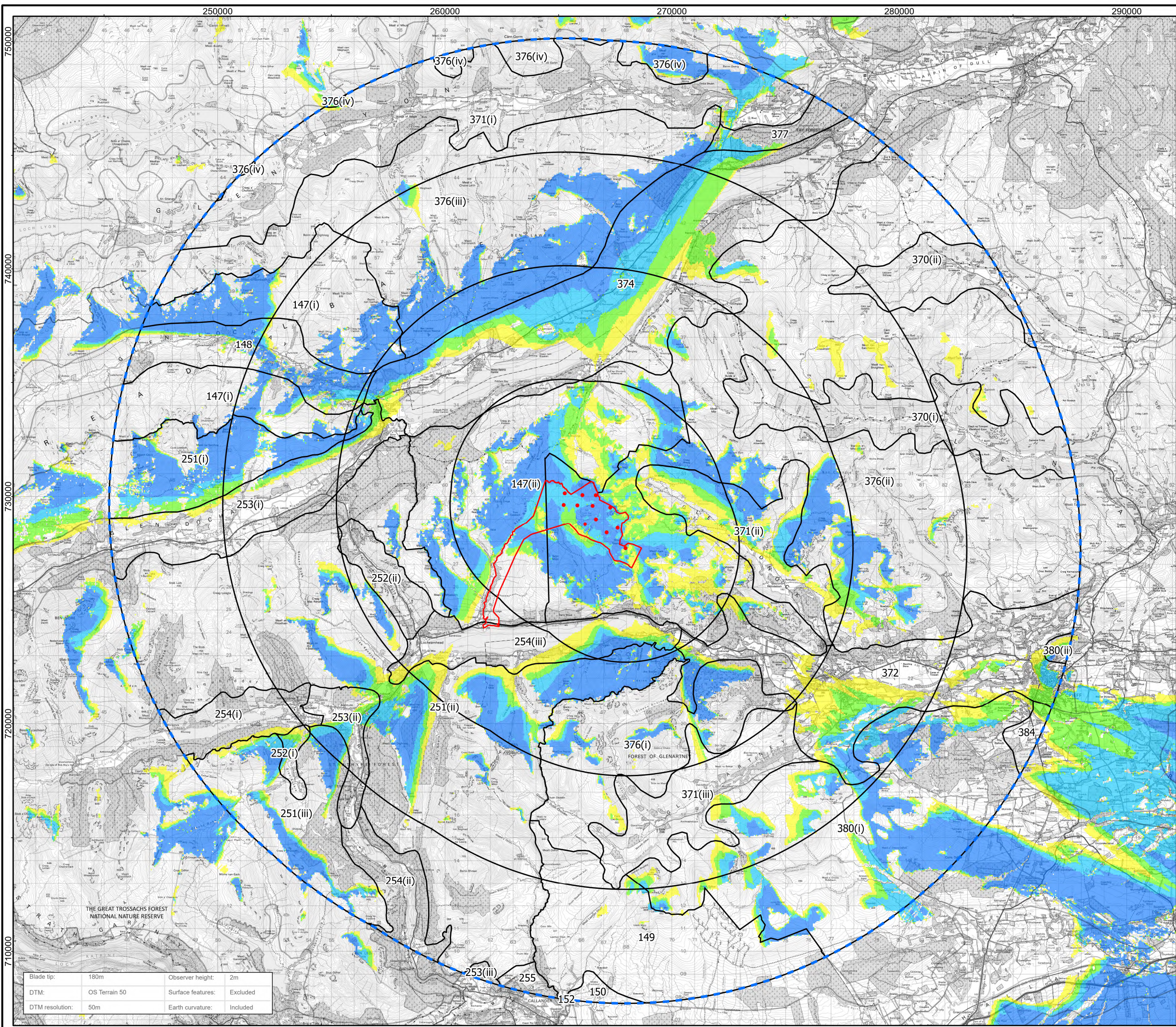
Figure 5.10 Landscape Character and Blade Tip ZTV Glentarken Wind Farm EIAR 2024
