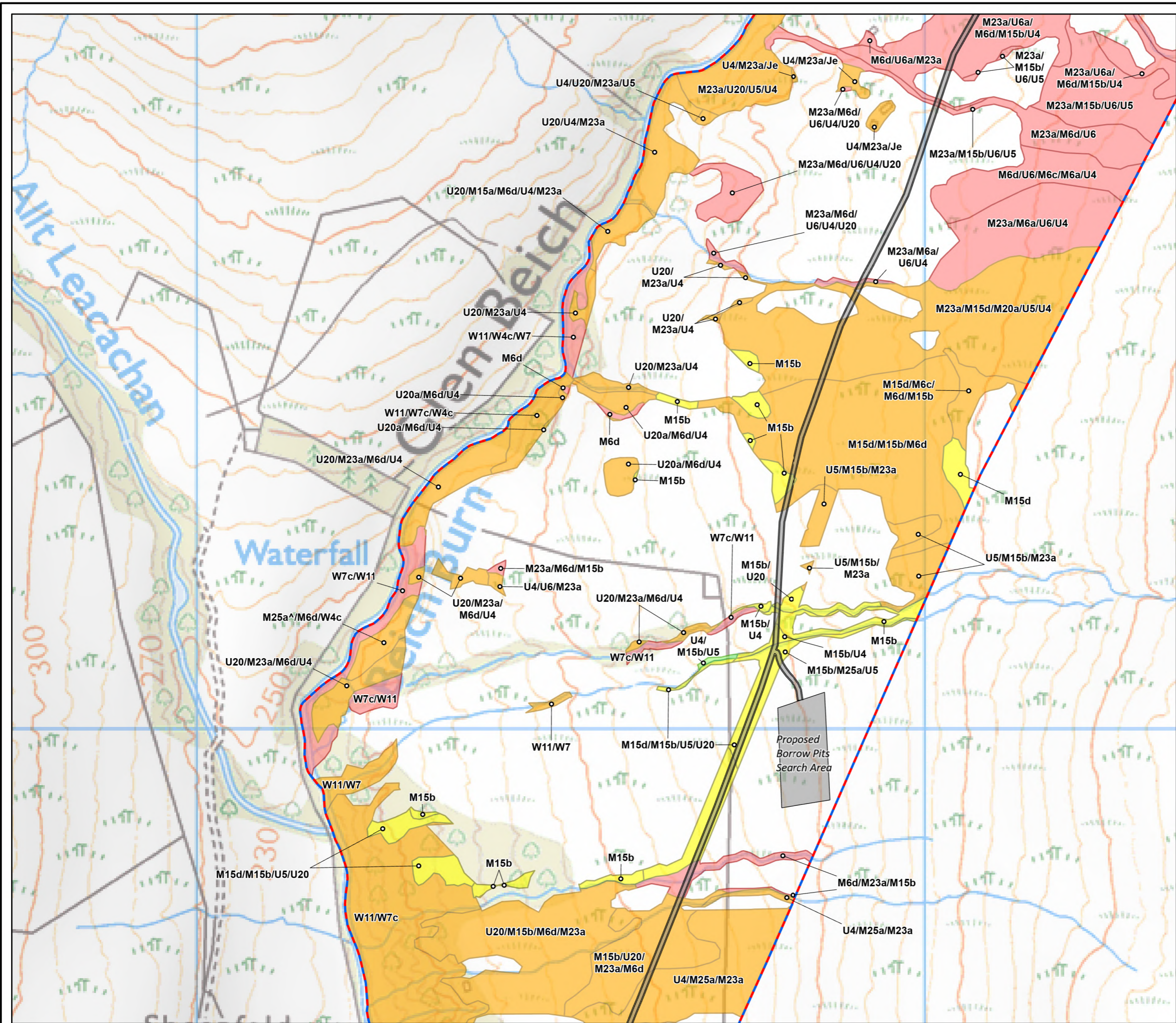
Figure 7.4.3 Potential Groundwater Dependent Terrestrial Ecosystems (GWDTEs) Glentarken Wind Farm EIAR 2024
