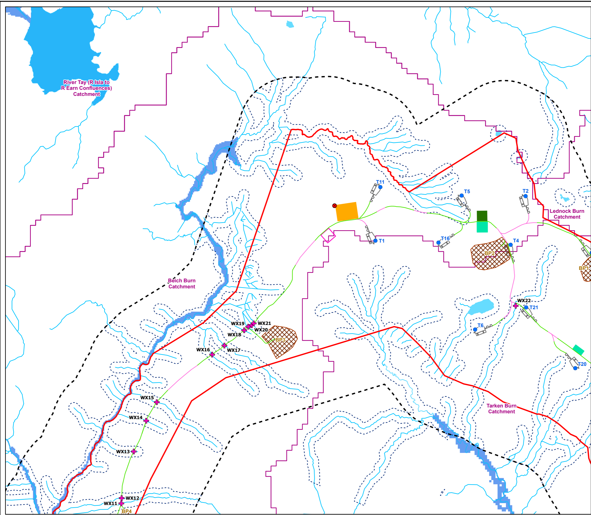
Figure 8.1c Local Hydrology
