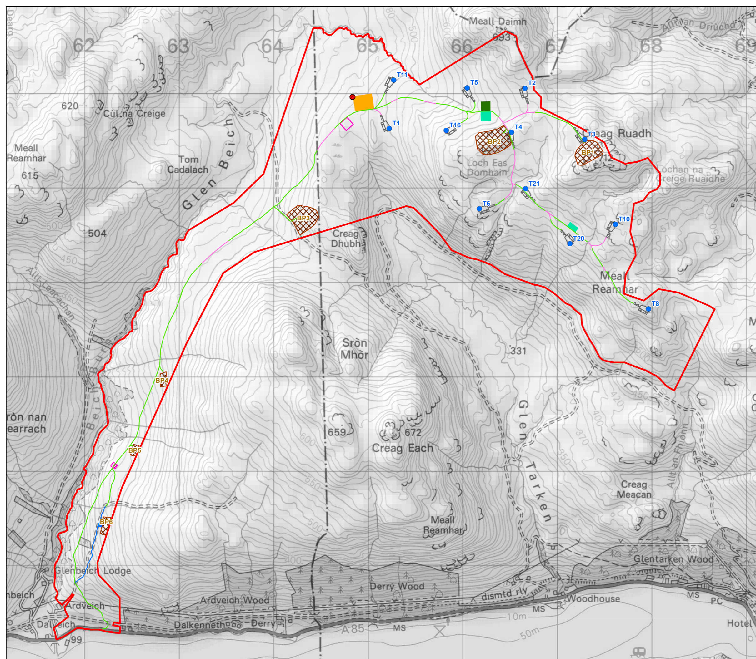
Figure 8.3.1 Borrow Pit Assessment: Site Layout Glentarken Wind Farm EIAR 2024
