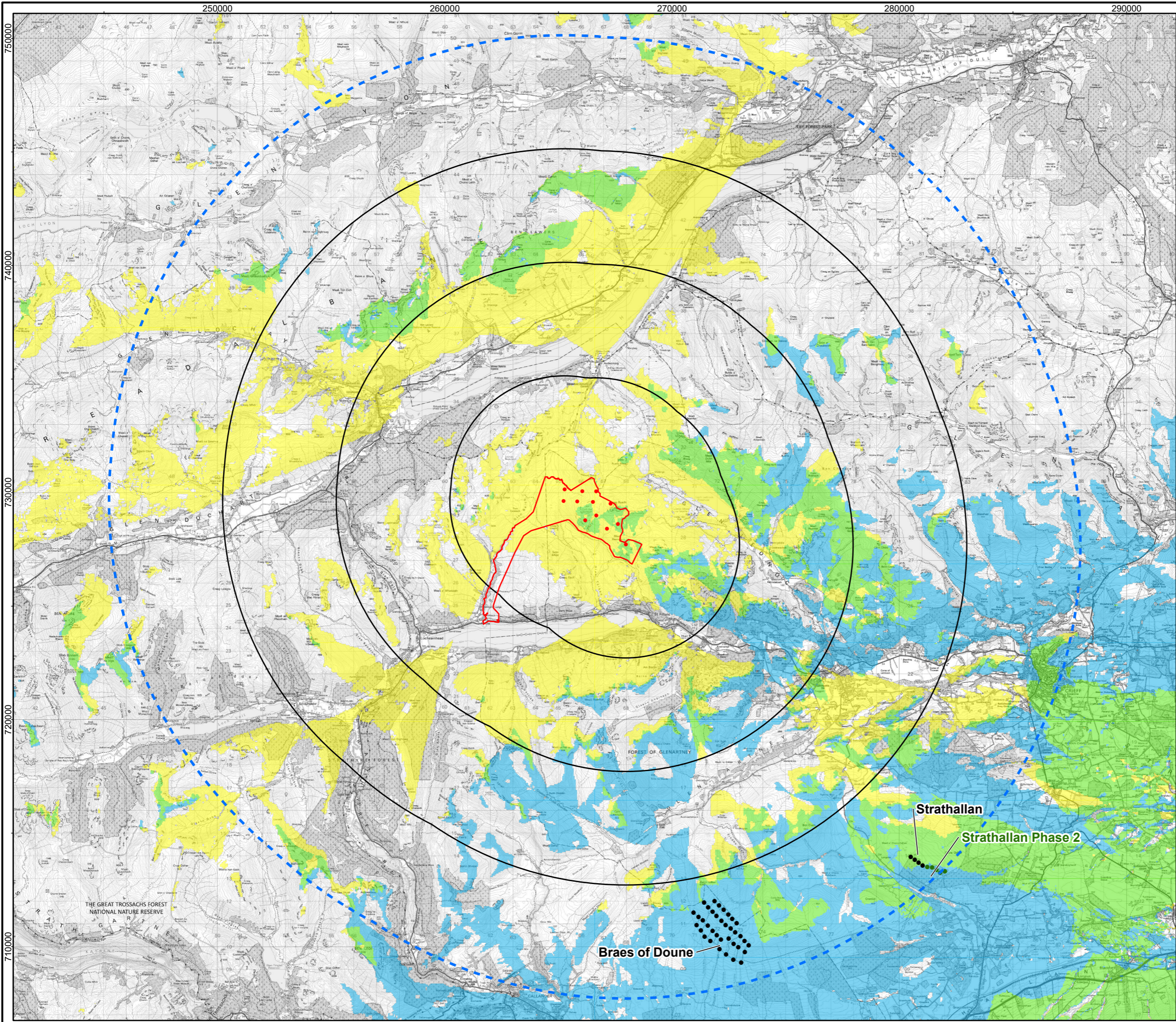
Figure 5.16b CZTV: Operational and Consented within 20 km + Proposed Development Glentarken Wind Farm EIAR 2024
