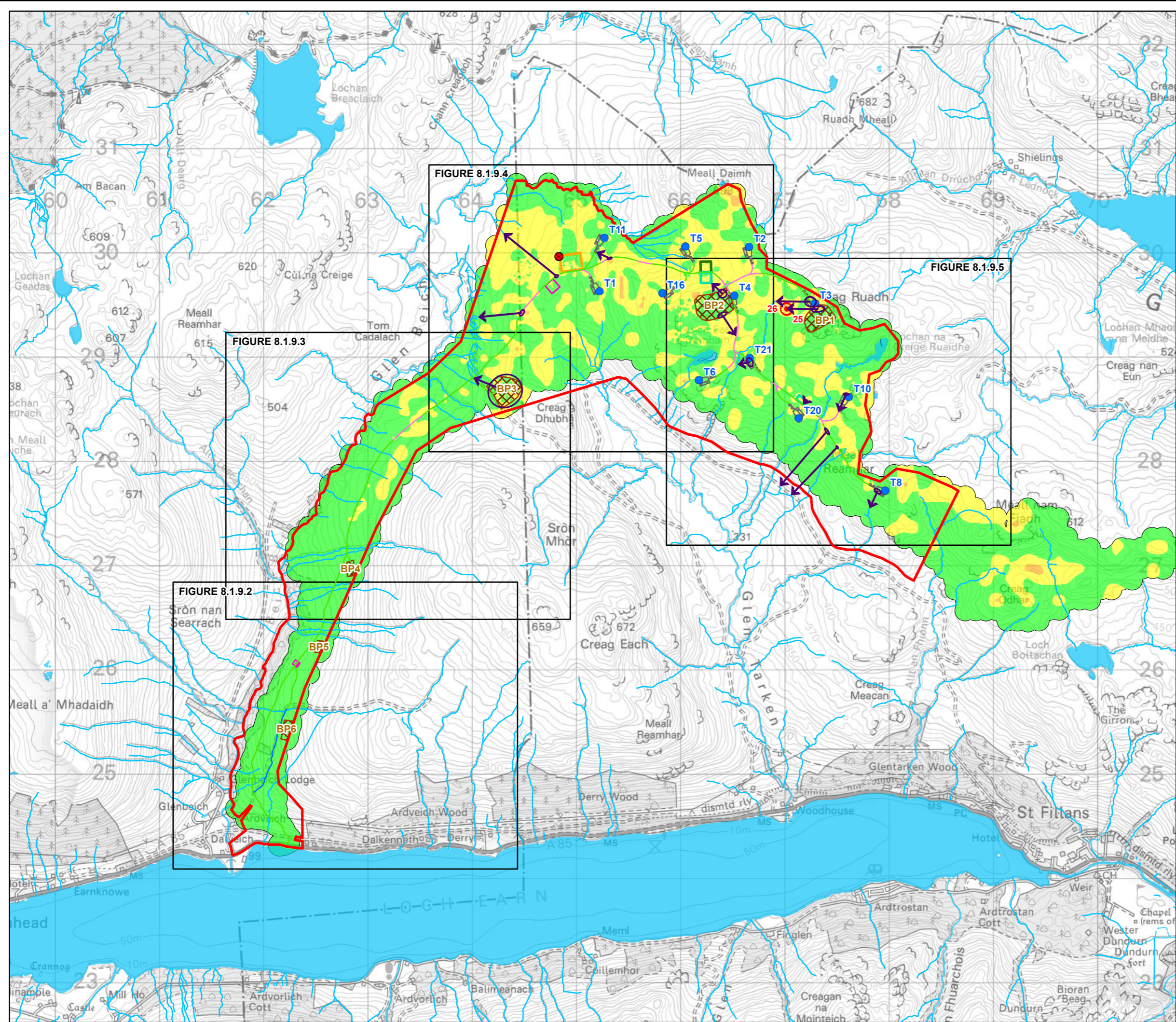
Figure 8.1.9.1 Peat Landslide and Hazard Risk Assessment: Slide Risk Glentarken Wind Farm EIAR 2024
