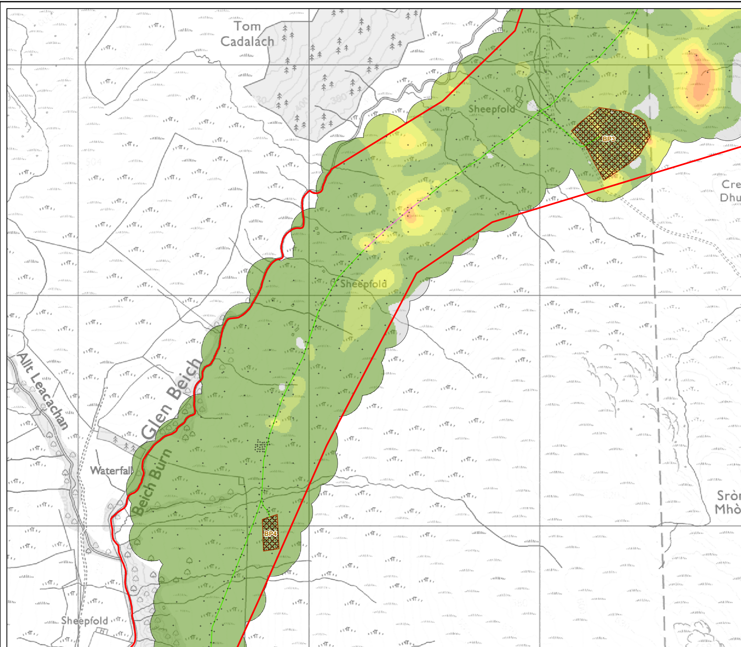
Figure 8.1.6.3 Peat Landslide and Hazard Risk Assessment: Peat Depth Plan Glentarken Wind Farm EIAR 2024
