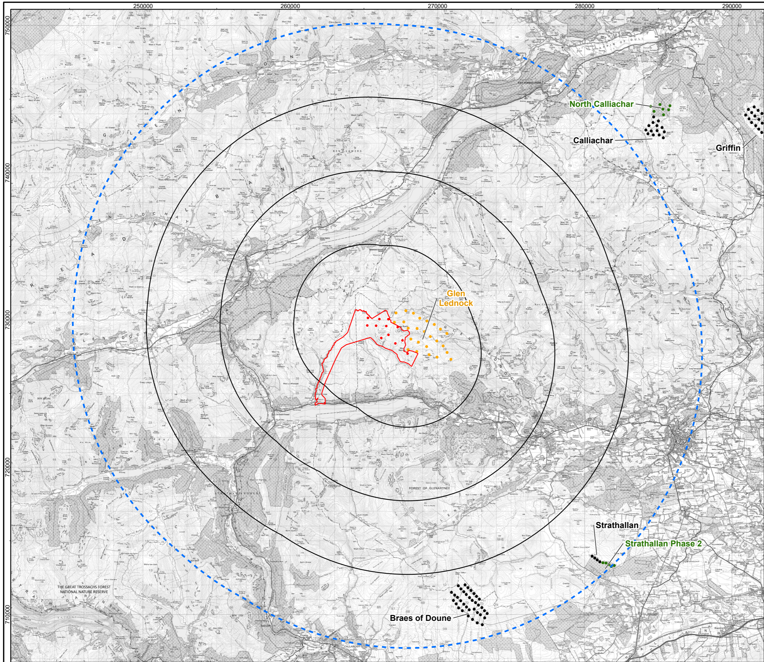
Figure 5.15 Cumulative wind farms within 20 km Glentarken Wind Farm EIAR 2024
