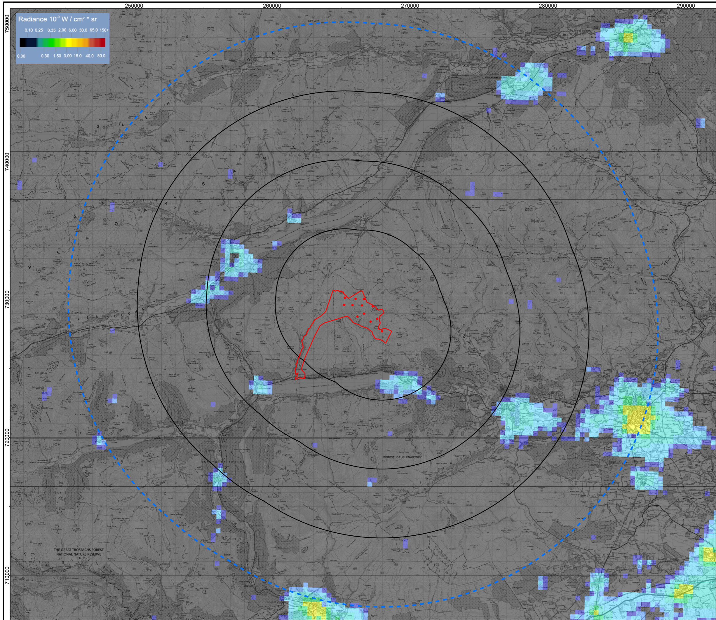
Figure 5.2.1 Baseline Light Pollution Glentarken Wind Farm EIAR 2024
