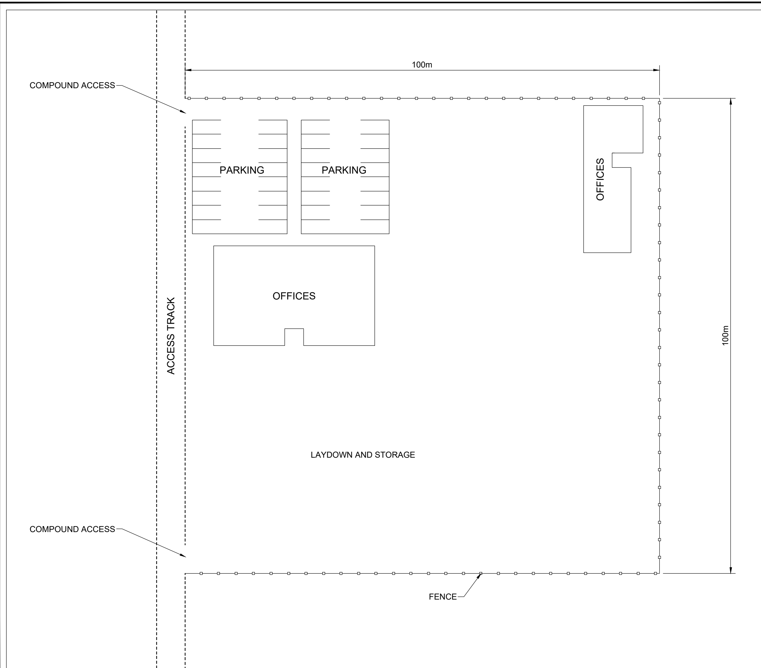
Figure 2.13 Typical Temporary Construction Compound Layout
