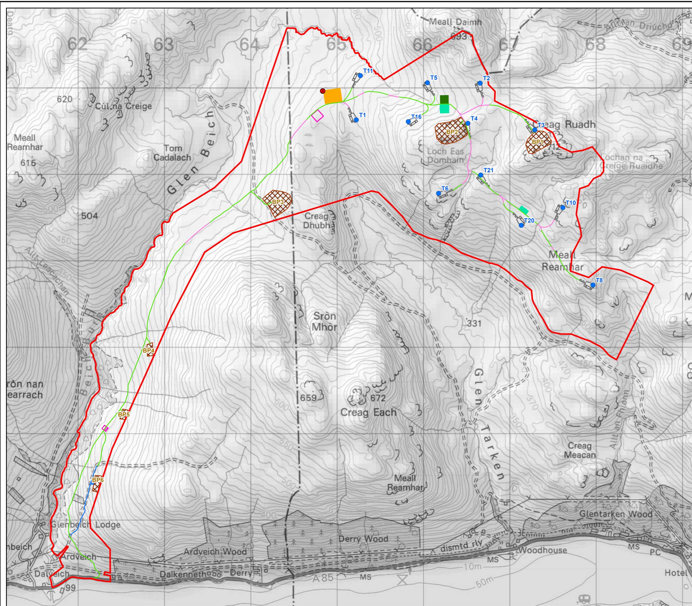
Figure 8.1.2 Peat Landslide and Hazard Risk Assessment: Site Layout Glentarken Wind Farm EIAR 2024
