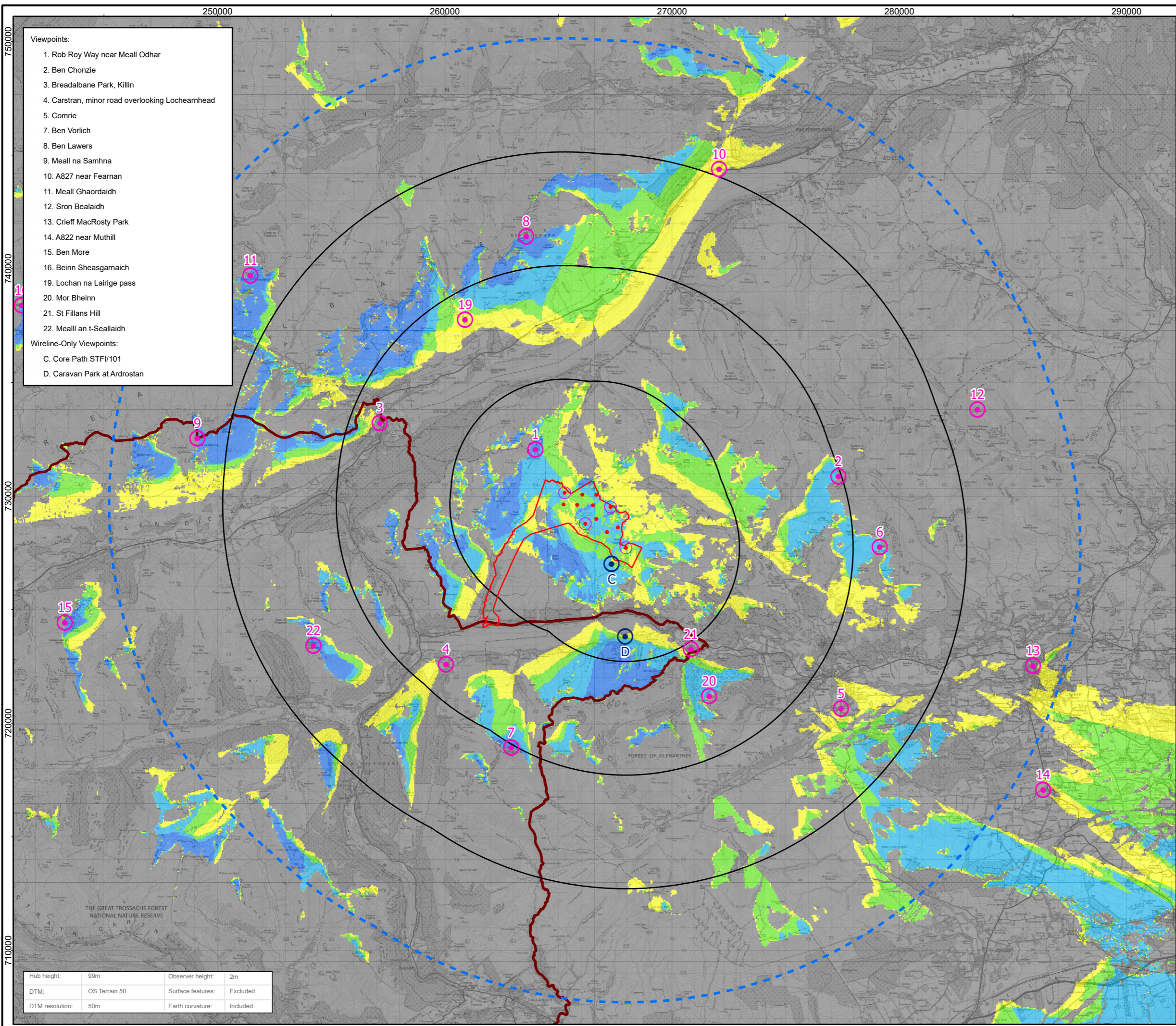
Figure 5.2.2 ZTV of Turbine Hub Lighting (reduced aviation lighting scheme) Glentarken Wind Farm EIAR 2024
