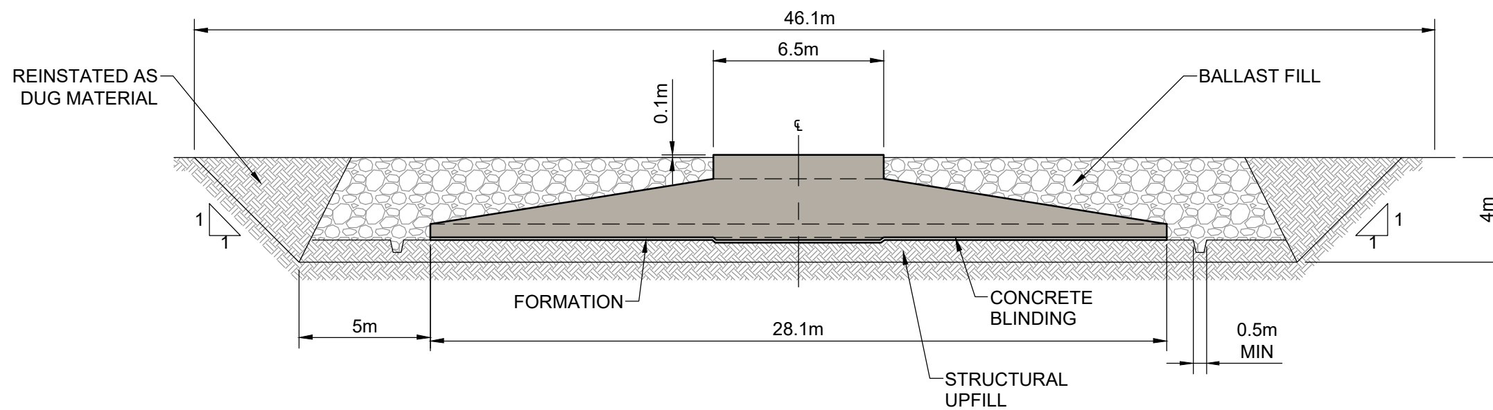
SECTION THROUGH TURBINE FOUNDATION Scale: 1:200
