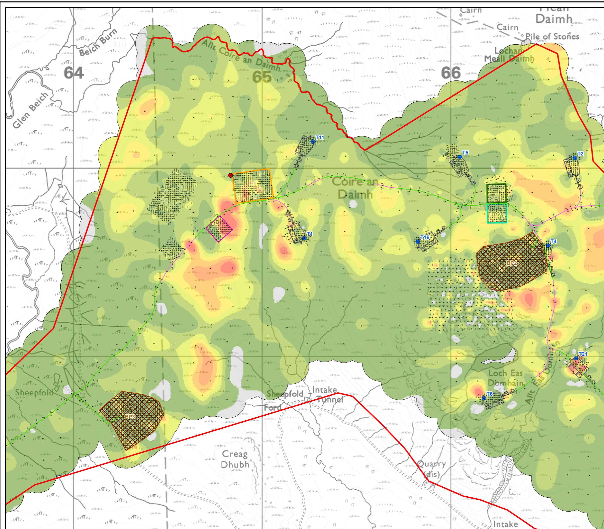
Figure 8.2.3.4 Peat Management Plan: Peat Depth Plan Glentarken Wind Farm EIAR 2024
