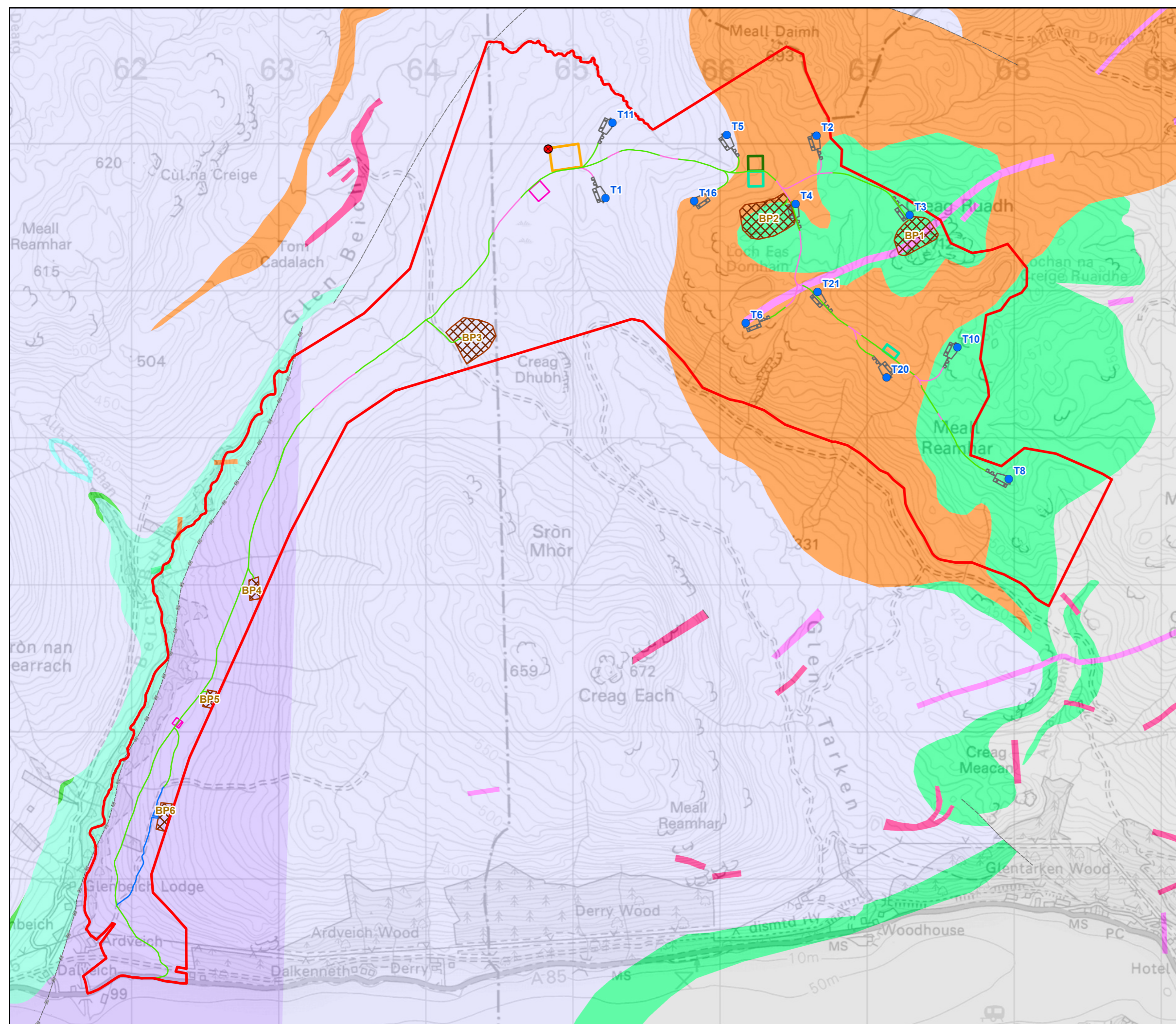
Figure 8.3.3a Borrow Pit Assessment: Bedrock Geology Glentarken Wind Farm EIAR 2024
