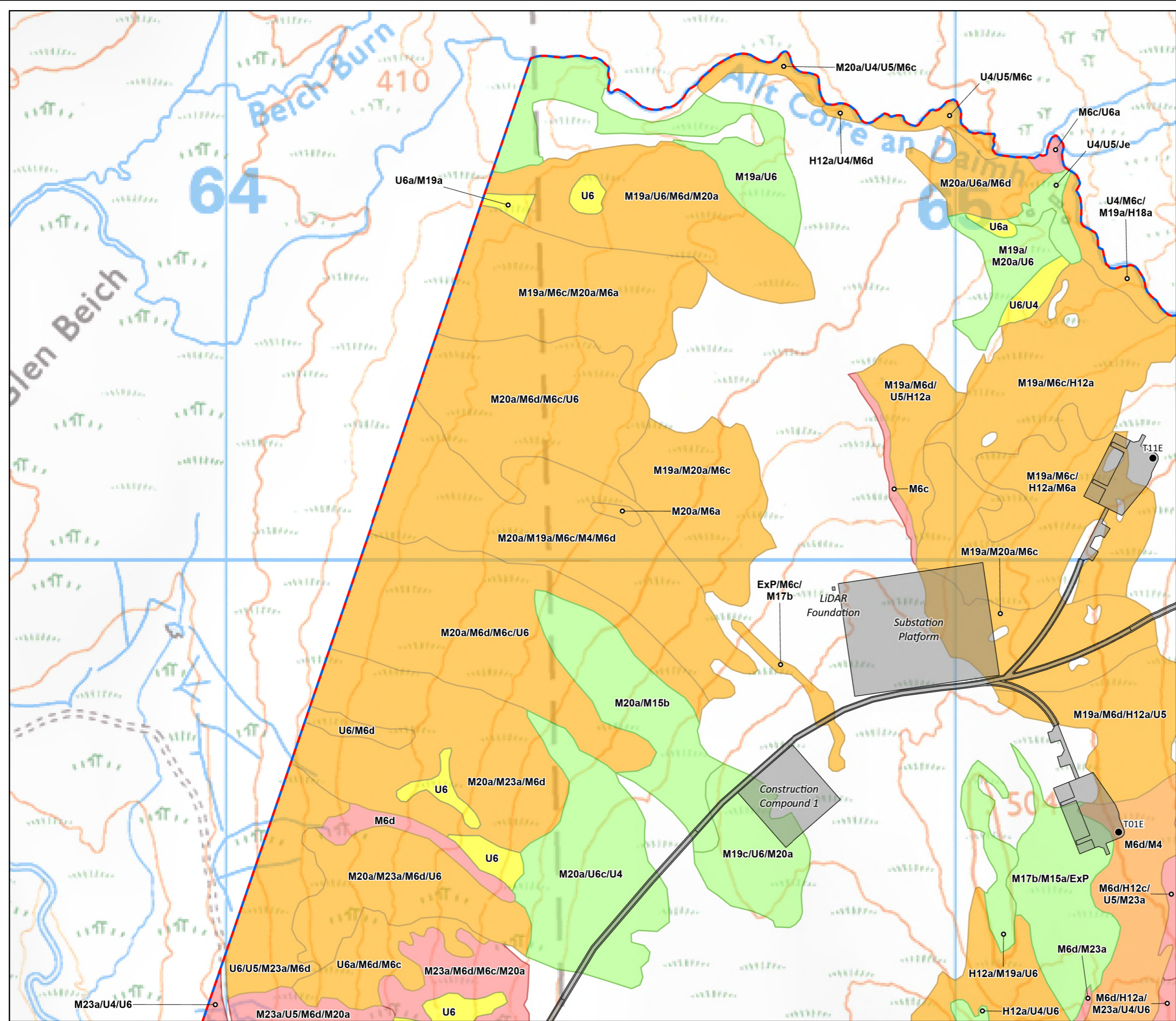
Figure 7.4.7 Potential Groundwater Dependent Terrestrial Ecosystems (GWDTEs) Glentarken Wind Farm EIAR 2024
