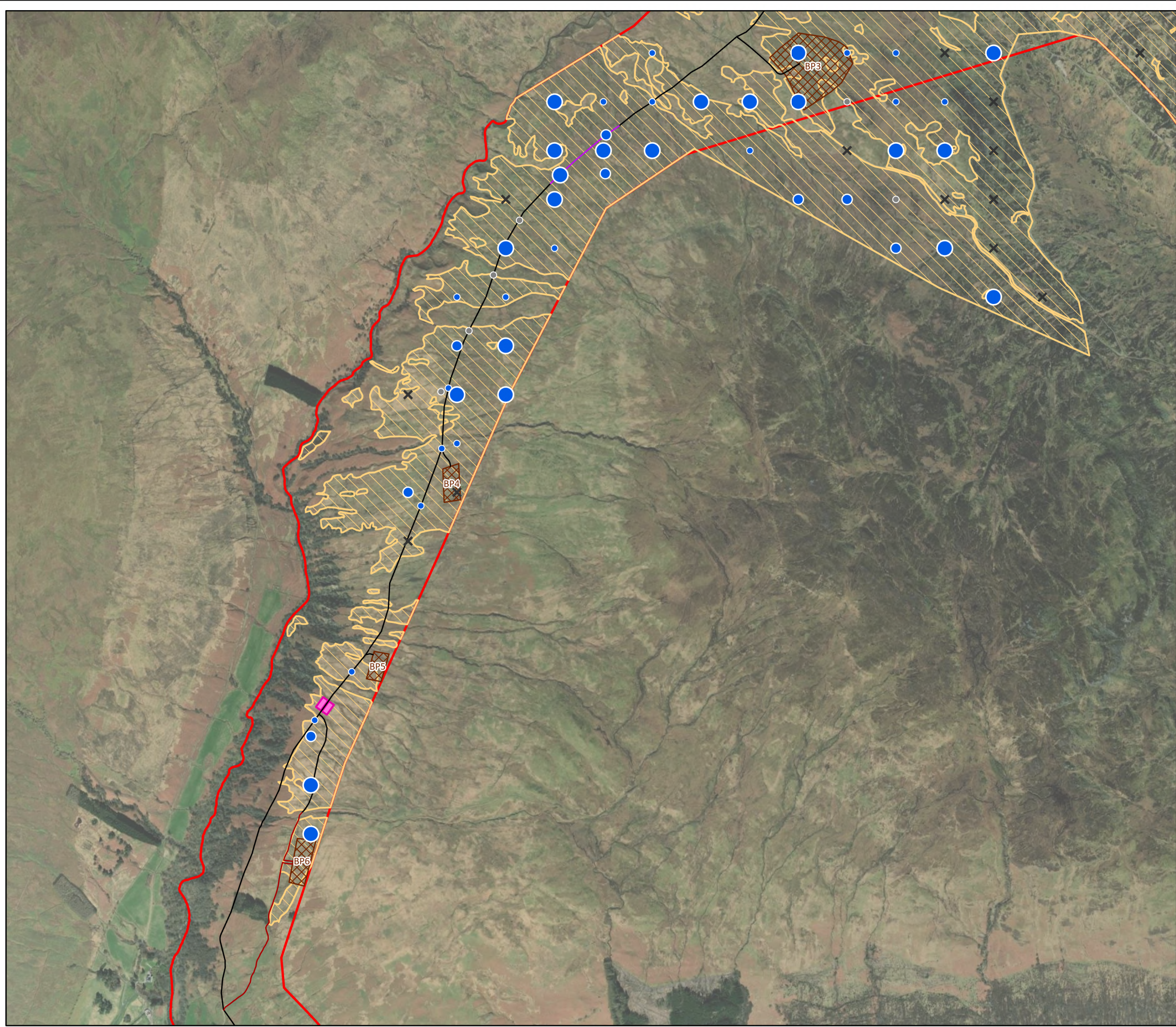
Figure 7.8.1 Sphagna Abundance and Distribution Glentarken Wind Farm EIAR 2024
