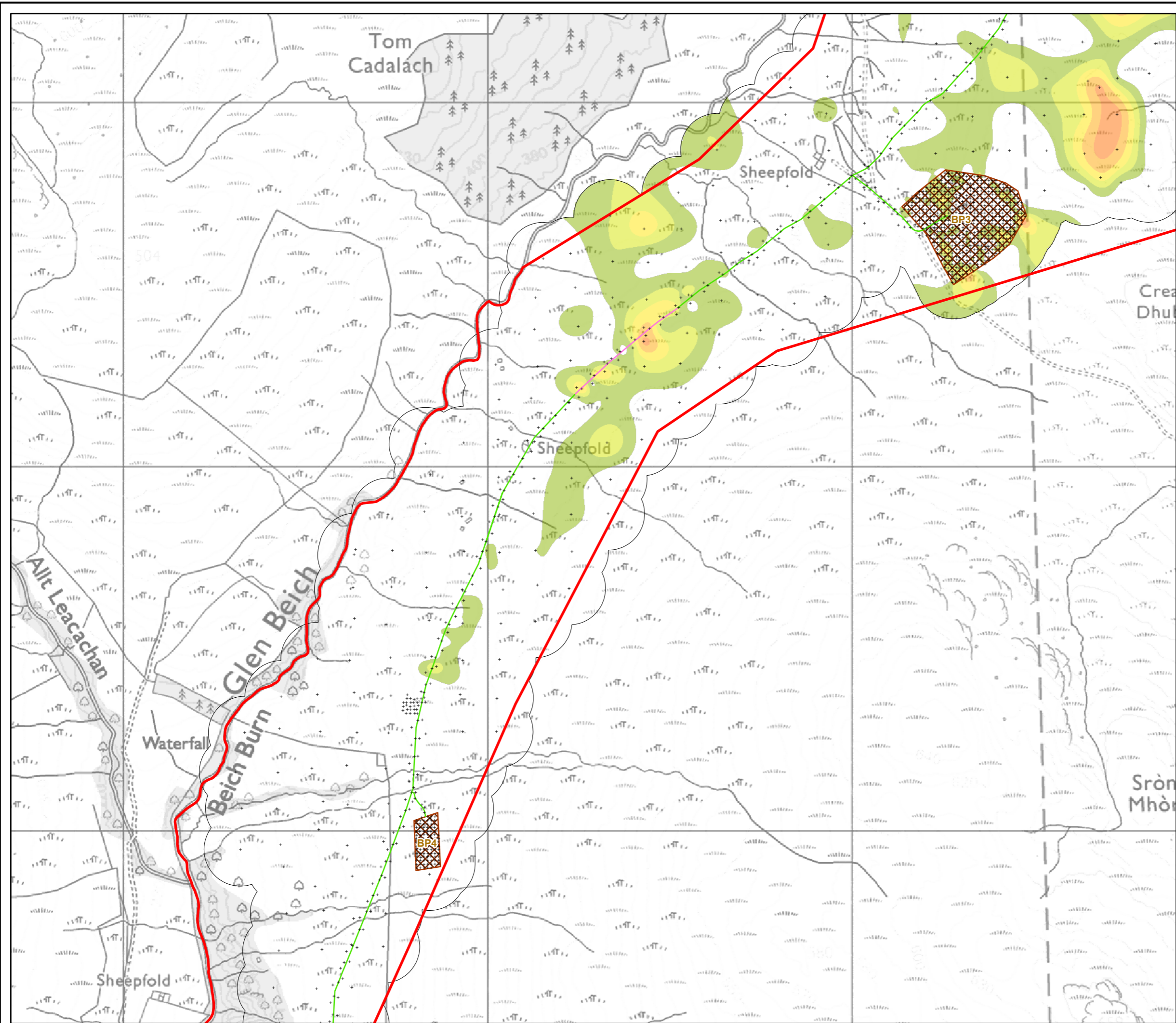
Figure 8.1.7.3 Peat Landslide and Hazard Risk Assessment: Peat Depth Over 0.5 m Glentarken Wind Farm EIAR 2024
