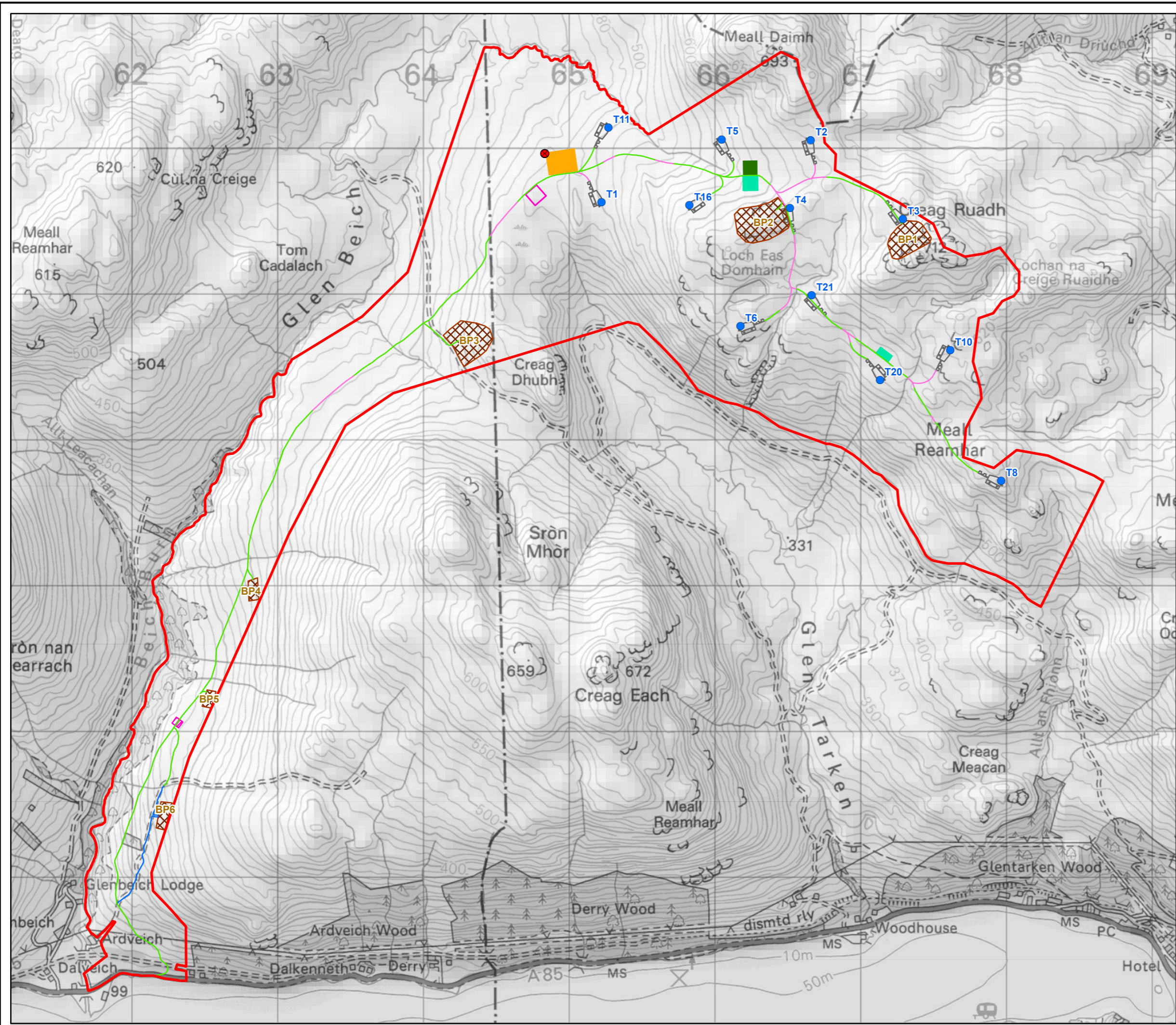
Figure 8.2.2 Peat Management Plan: Site Layout Glentarken Wind Farm EIAR 2024
