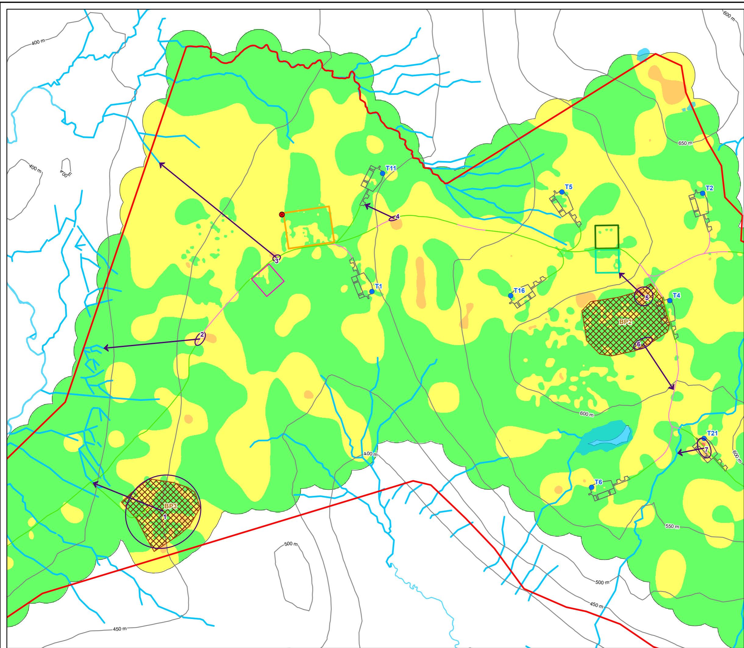
Figure 8.1.9.4 Peat Landslide and Hazard Risk Assessment: Slide Risk Glentarken Wind Farm EIAR 2024
