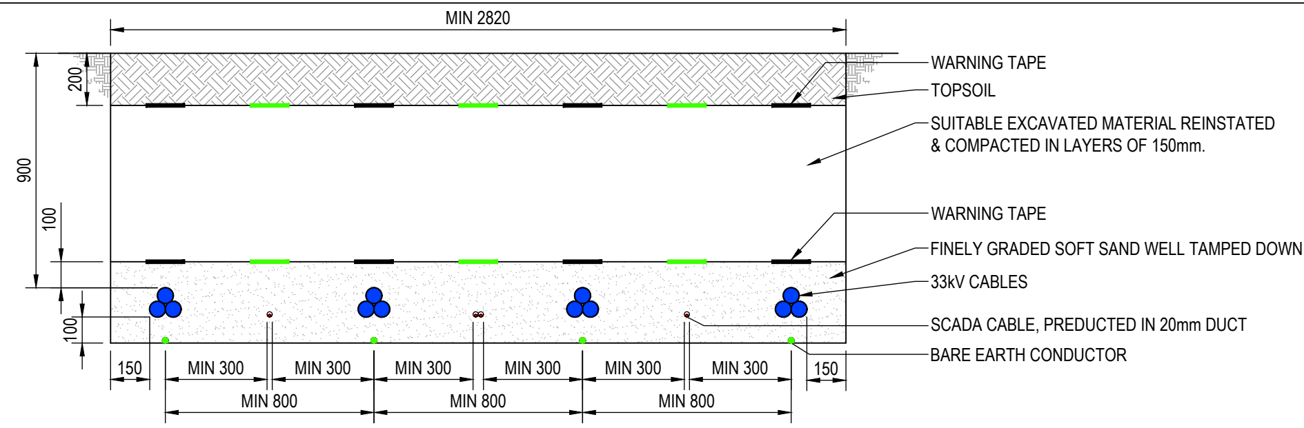
TYPICAL 33kV FOUR CIRCUIT CABLE TRENCH DIRECT BURIED
