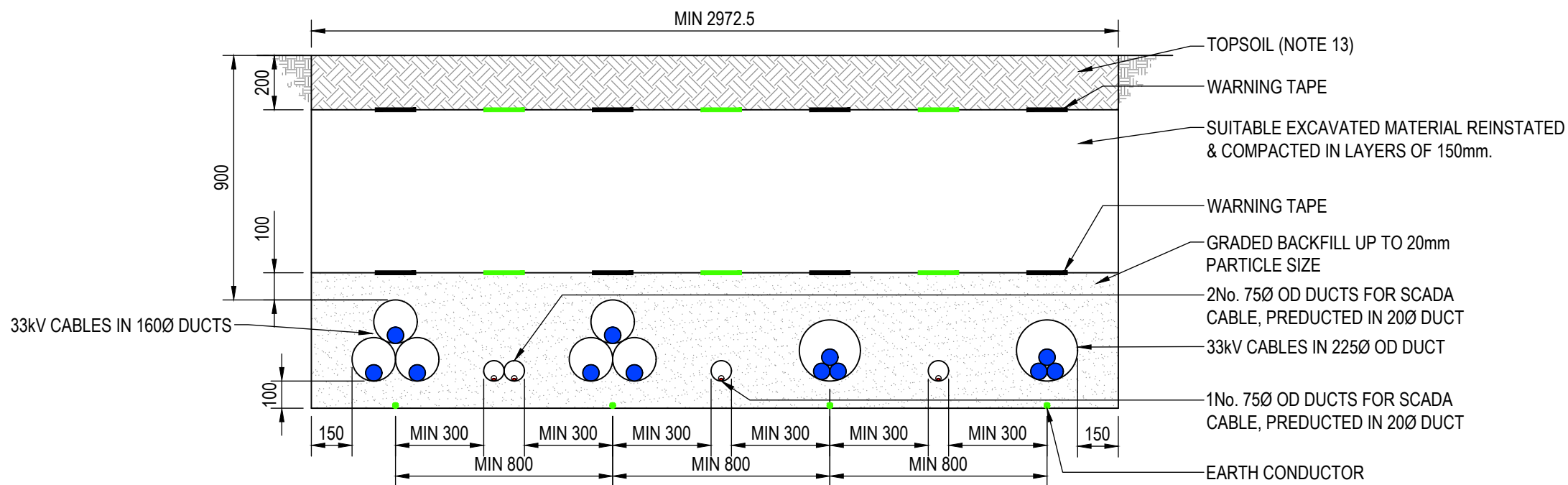
TYPICAL 33kV FOUR CIRCUIT DUCT LAYOUT IN TRENCH
