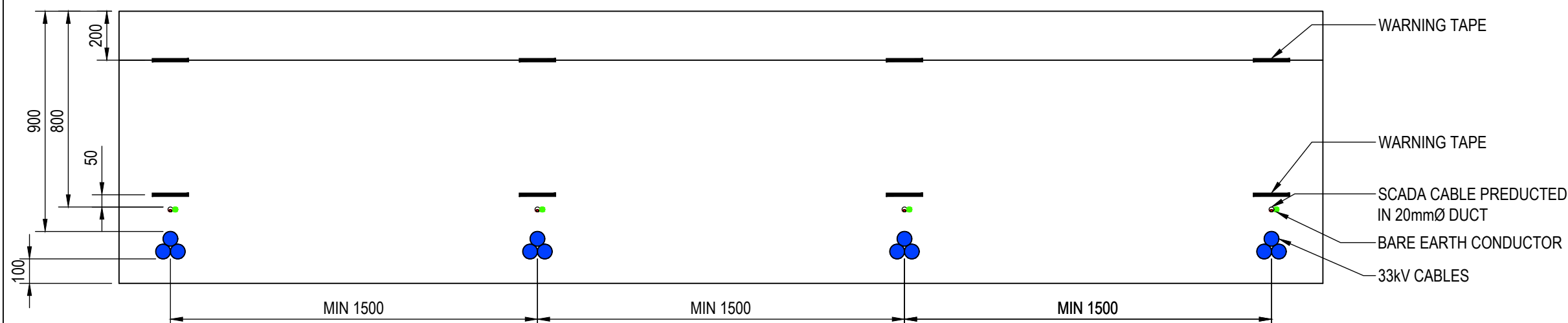
TYPICAL 33kV FOUR CIRCUIT PLOUGHED CABLE TRENCH
