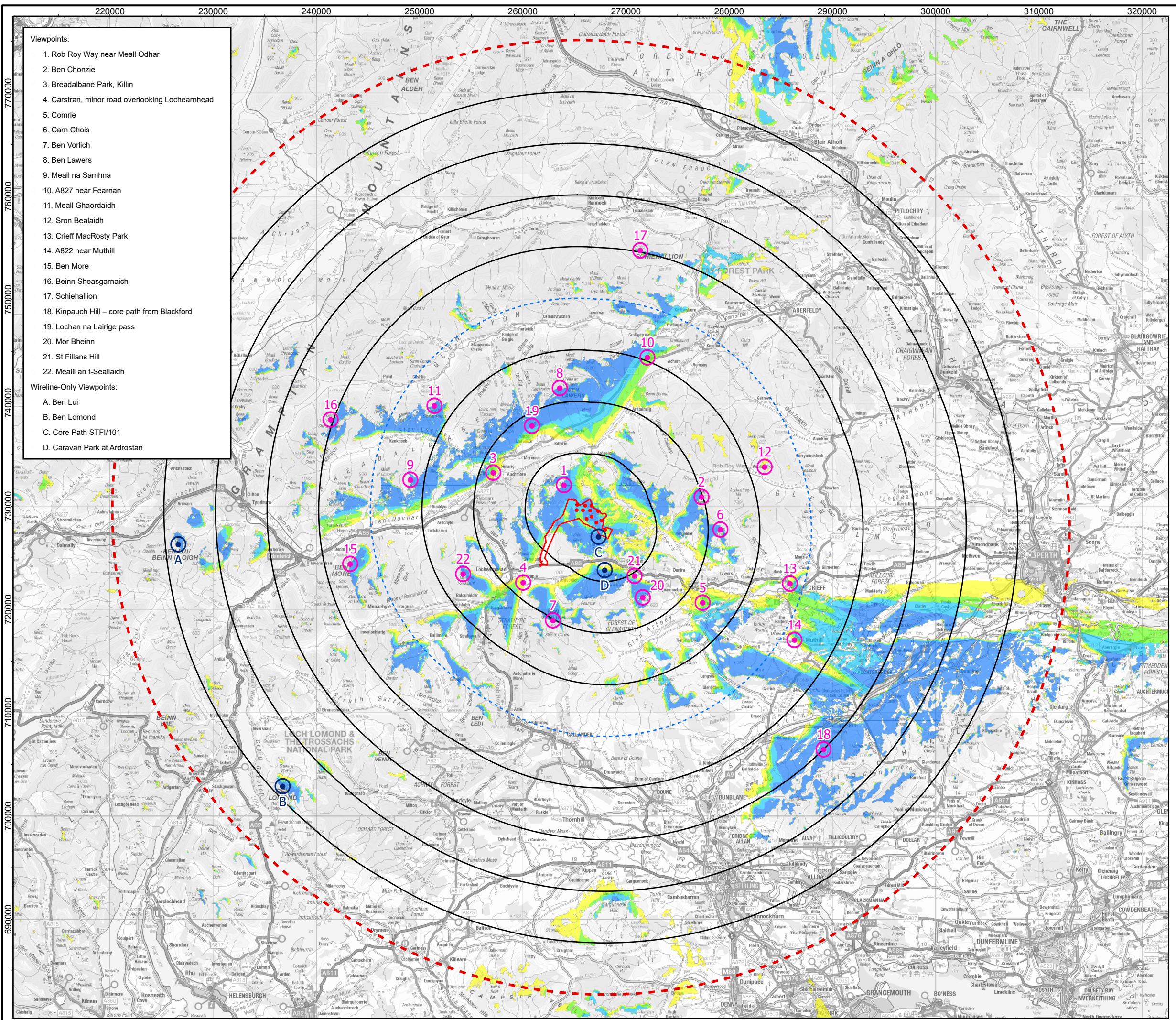
Figure 5.7a Blade tip ZTV with viewpoints (A3) Glentarken Wind Farm EIAR 2024
